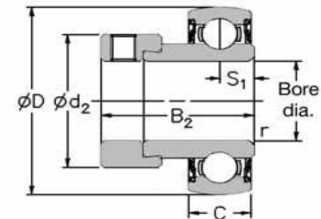
1200EC With spherical outside diameter, non-regreaseable outer ring and eccentric locking collar
