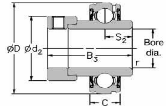
1000DECG With spherical outside diameter and eccentric locking collar
